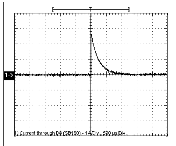
Figure 14 - Current Through SB160 Protection Diode
