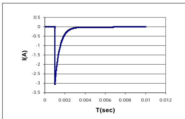
Figure 4 - Current through R S1 After S 1 Closes
