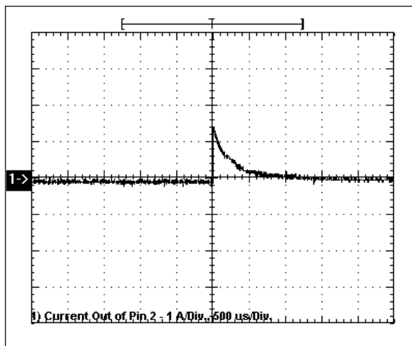
Figure 10 - Current Out of Pin 2 of Unprotected Mic Pre IC
