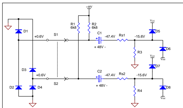
Figure 3 - Simulation Circuit Immediately After Switches Close
