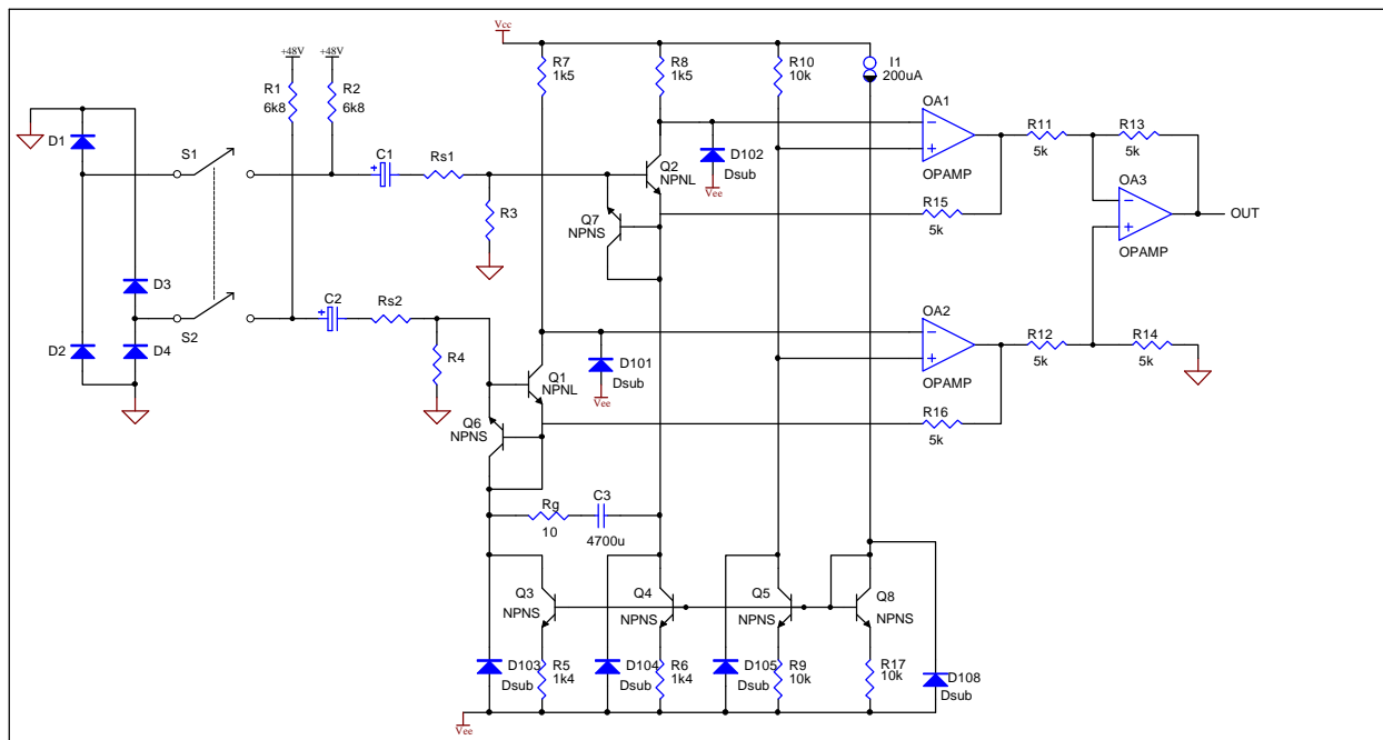
Figure 5 - Simulation Circuit Including Microphone Preampfier
