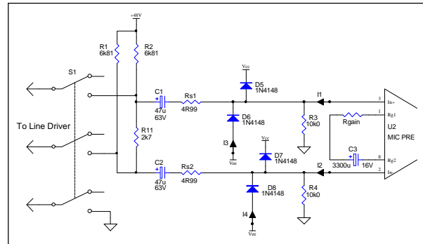
Figure 13 - Microphone Preamplifier IC with Diode Protection
