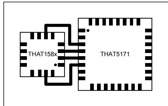
Figure 15. Recommended THAT158x/THAT5171 PCB Layout (mounted on same-side of PCB).
