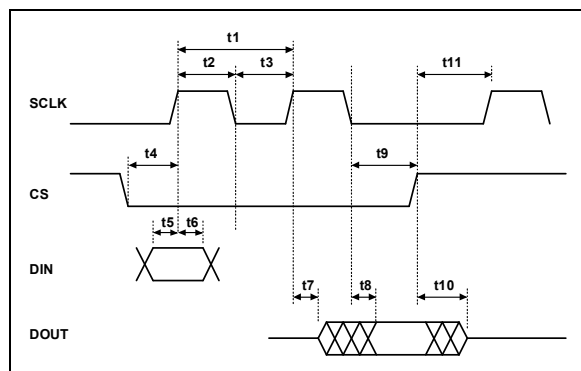
Figure 7. SPI Timing.
