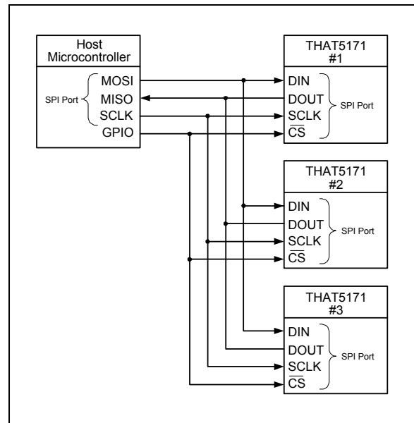
Figure 13. Multiple 5171 ICs connected in parallel to a host microcontroller.
