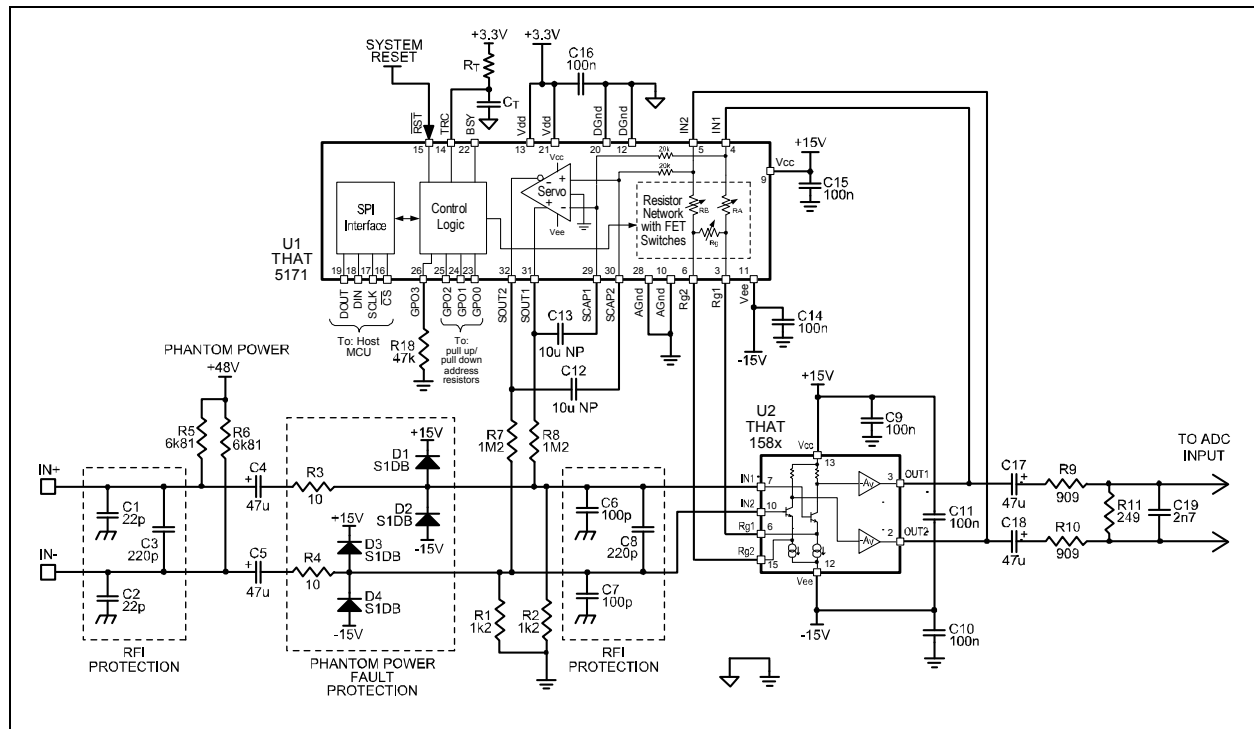
Figure 5. 5171/ 158x low-cost application for output to an A/D converter.
