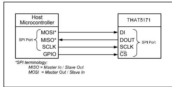
Figure 12. Single 5171 connected to a host microcontroller.
