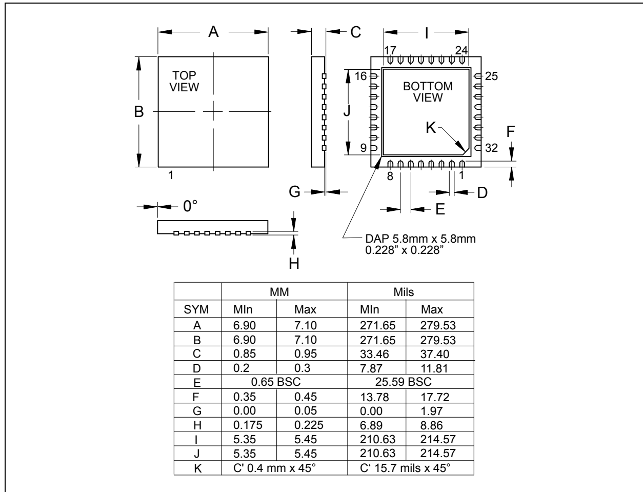
Figure 16. 7 x 7mm QFN32 Package Dimensions.
