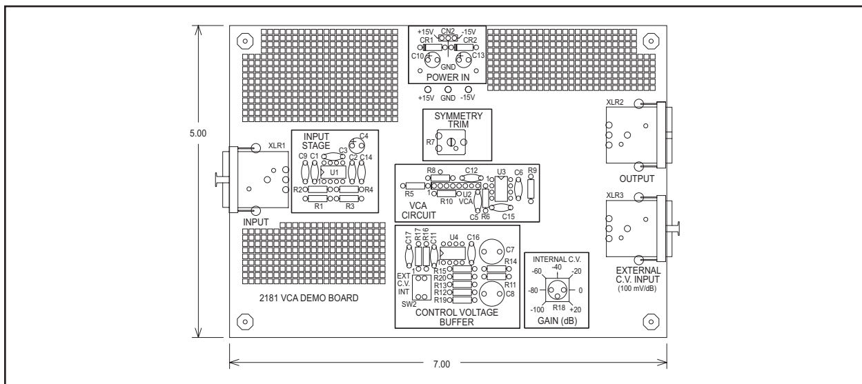
Figure 2. 2181-DEMO Outline Drawing
